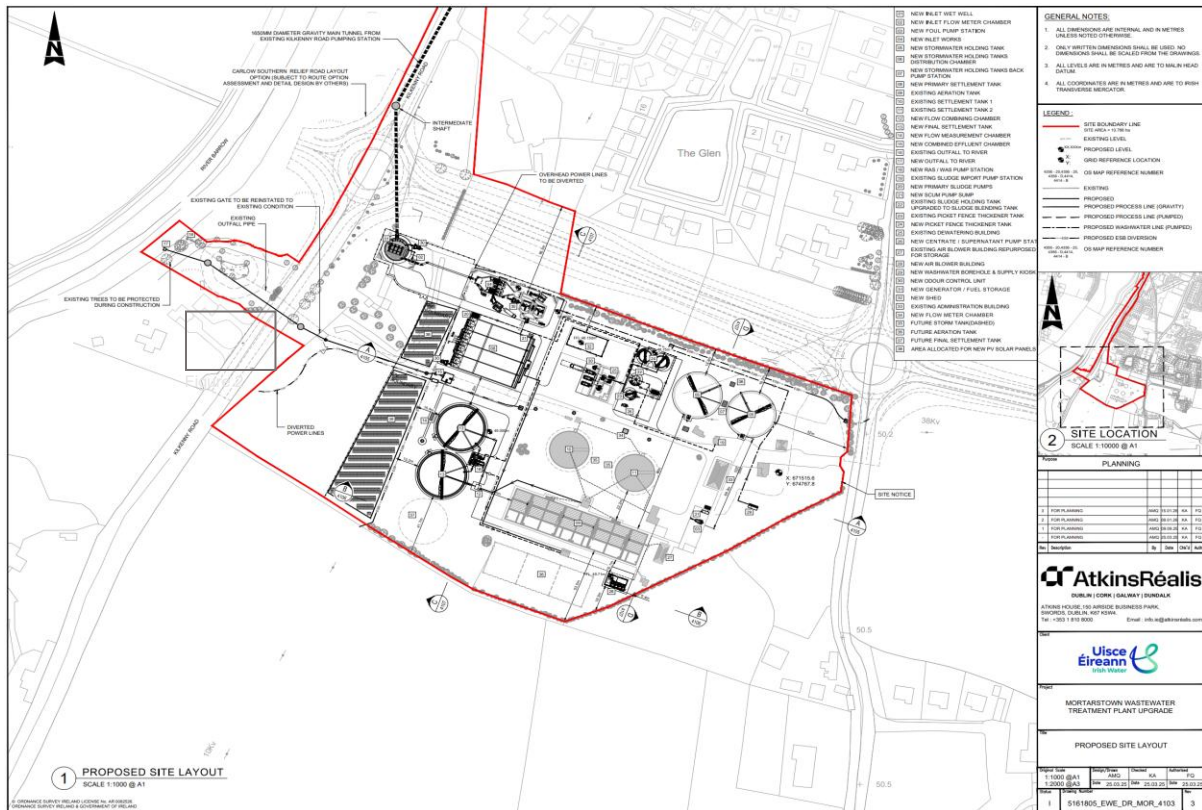
Figure 1 - Proposed Boundary of Site Works.
