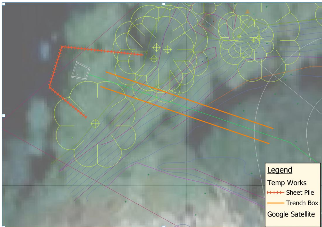
Figure 2 - Proposed location of sheet piles.
